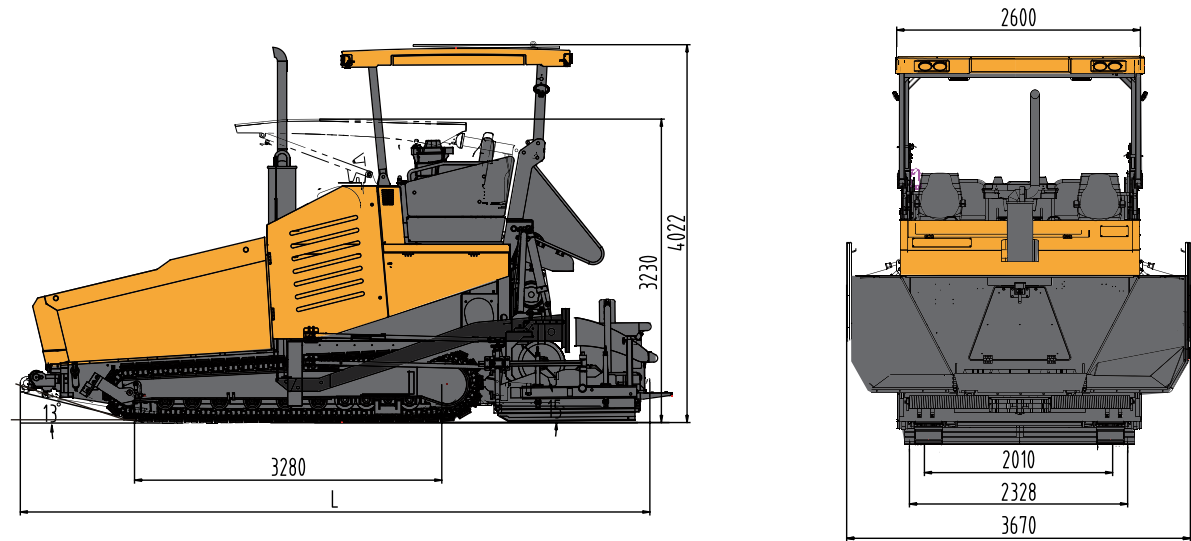
L 配 SF250 熨平板为 6710mm，配 SE570/470 熨平板为 7250mm 6710 mm screed equipped with SF250, and 7,250 mm screed equipped with SE570/470
